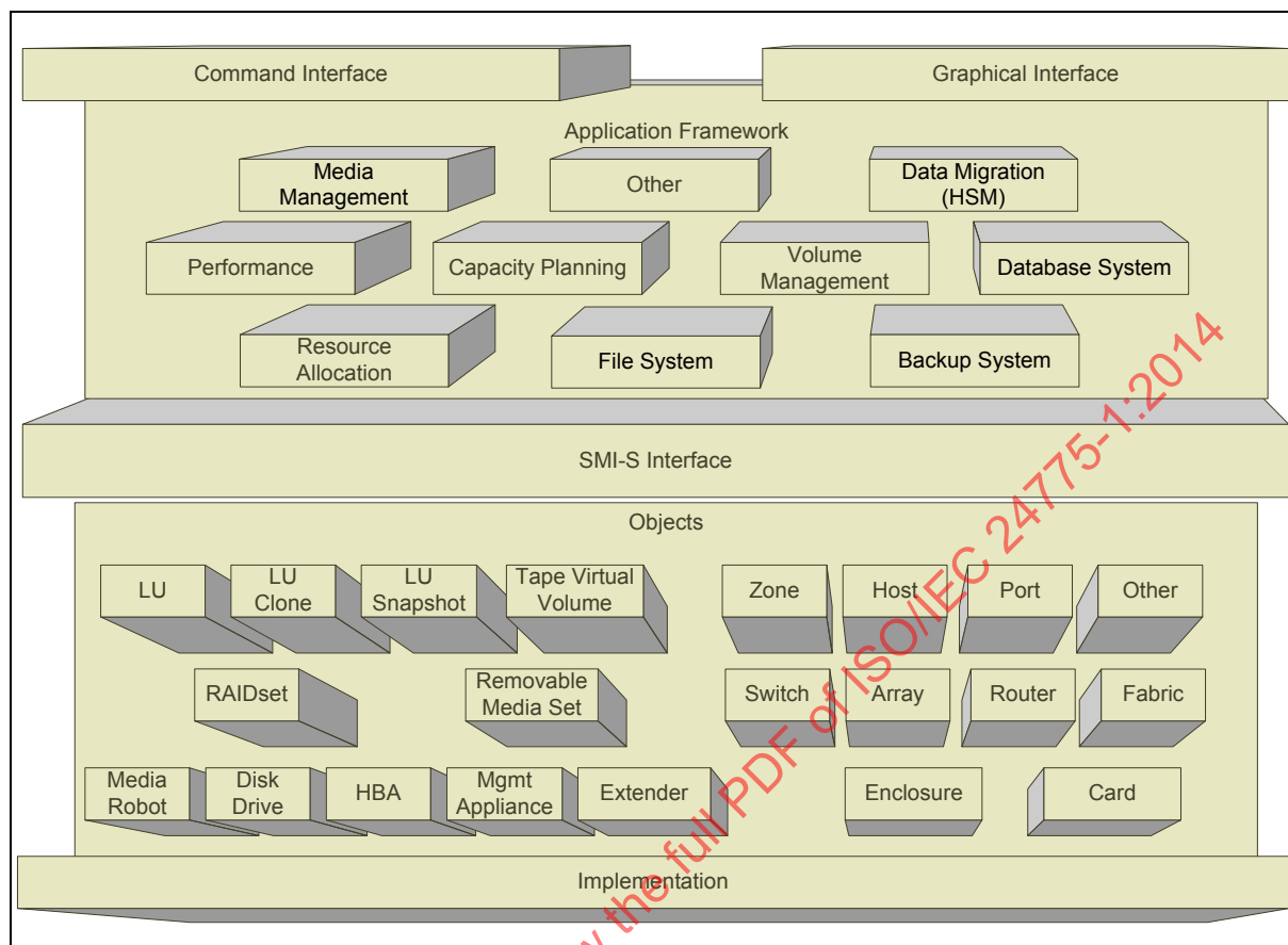
Figure 5 – Interface functions
