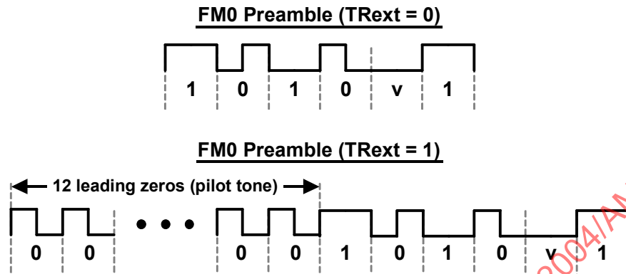
Figure Amd.1-14 — FM0 T=>R preamble
