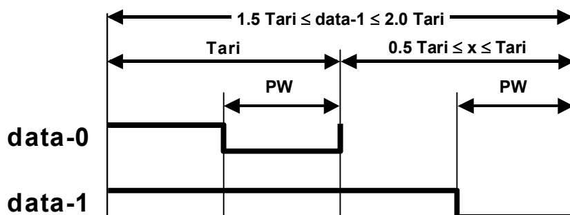
Figure Amd.1-4 — PIE Symbols
