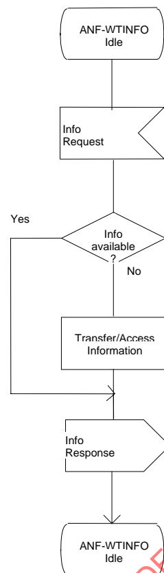
Figure 2: ANF-WTINFO, overall SDL diagram
