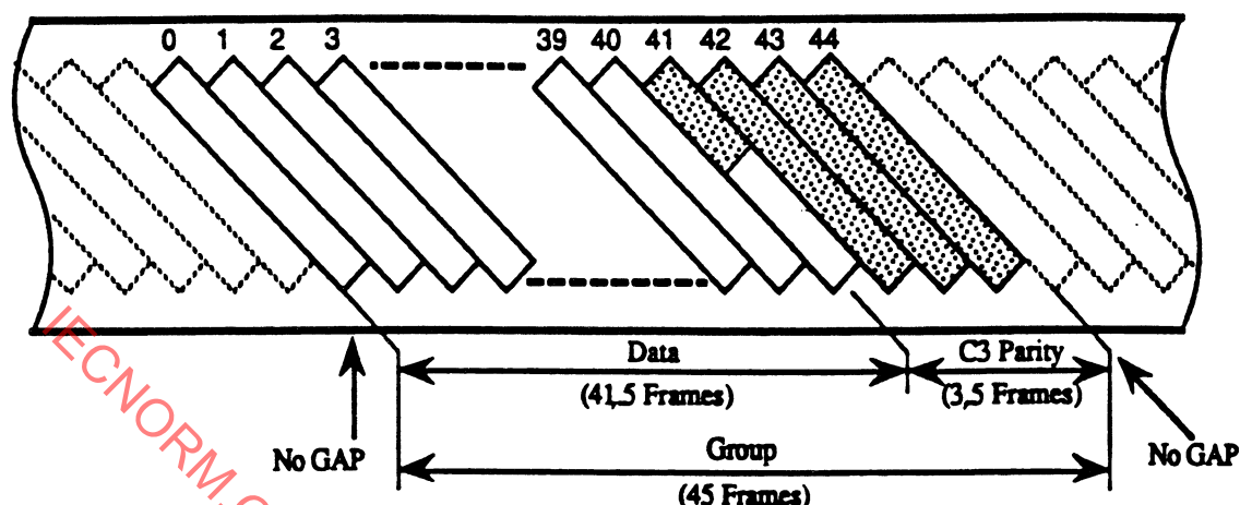
Figure 52 - Group Format 1
