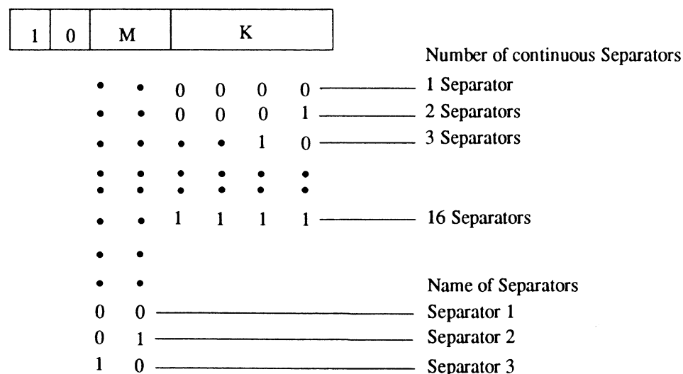
Figure 47 - Control Byte for Separators 1, 2 and 3
