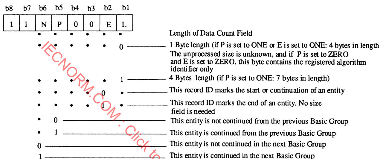
Figure 48 - Control Byte for entities
