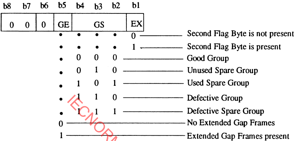
Figure 65 - First Flag Byte for Type A
