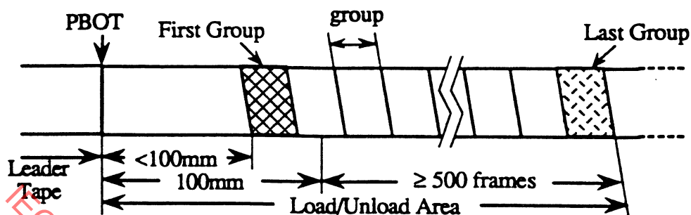
Figure 54 - Load/Unload Area
