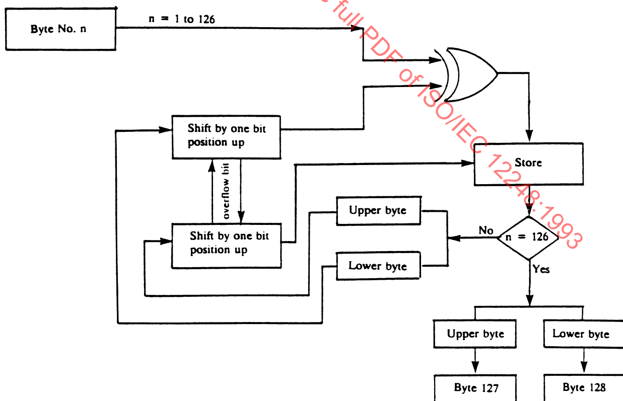
Figure 57 - Checksum summary
