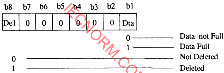
Figure 61 - Partition Flags
