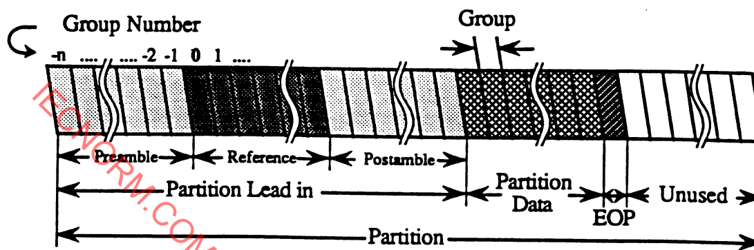
Figure 62 - Partition organization
