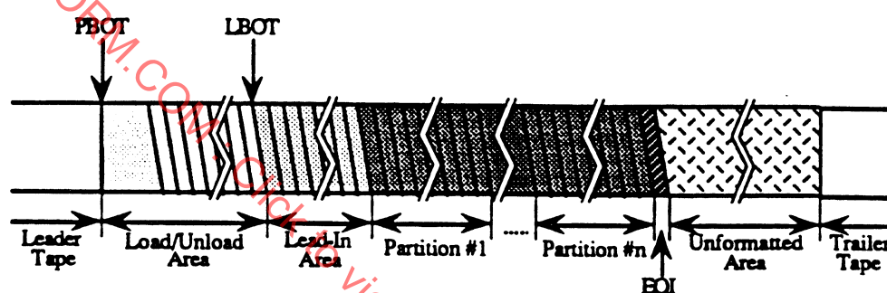
Figure 53 - Tape Format
