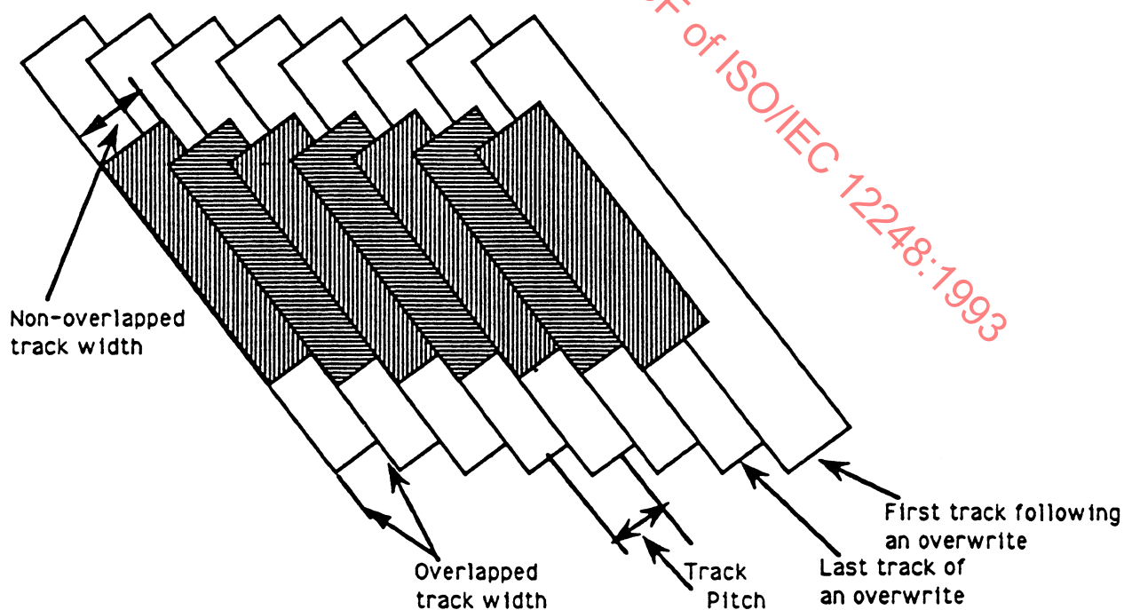
Figure 77 - Track configuration after overwrite
