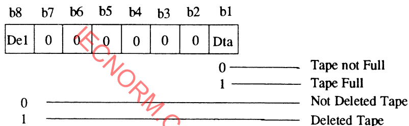
Figure 59 - Tape Flag
