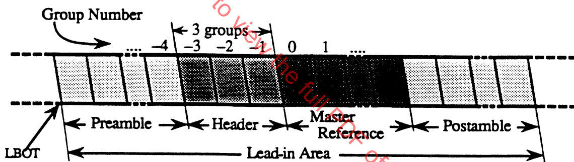
Figure 55 - Lead-in Area
