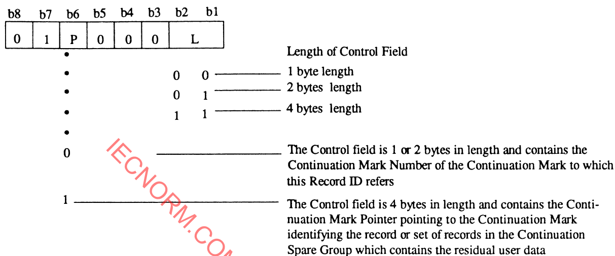
Figure 46. Control Byte for Continuation Marks
