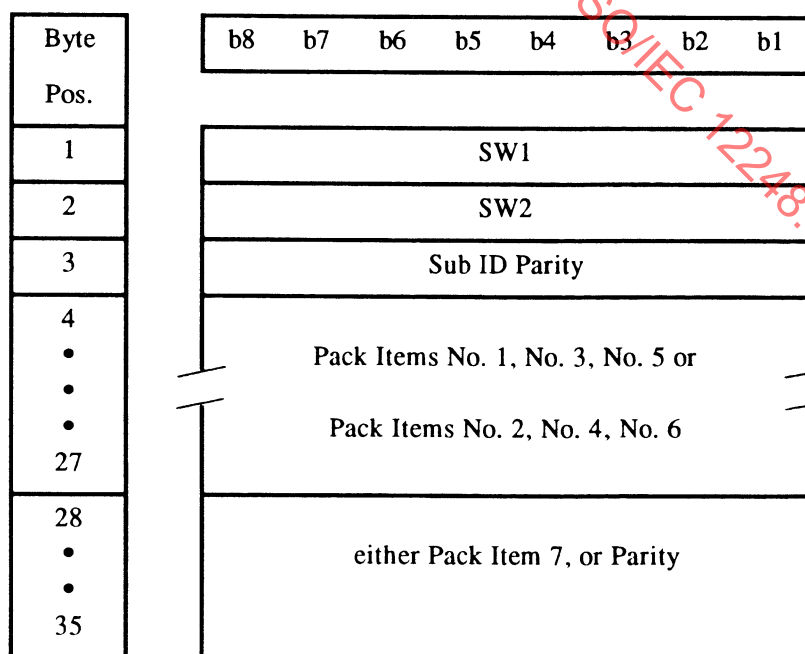
Figure 39 - Sub Data Block
