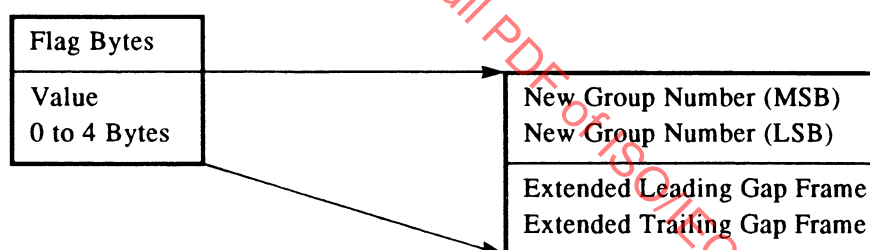
Figure 64 - Type A Group Entry
