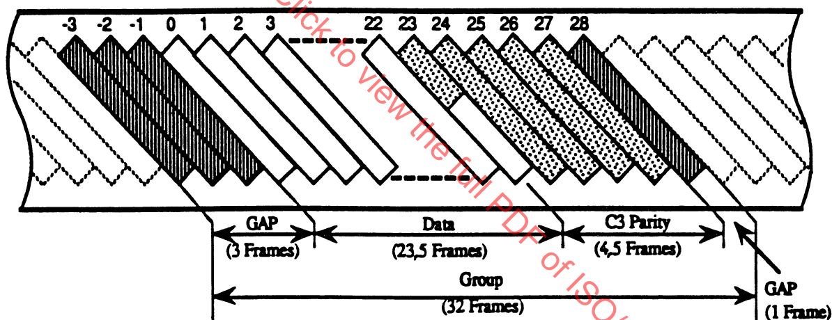
Figure 51 - Group Format 0
