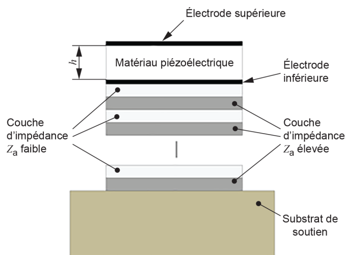
Figure 2 – Configuration SMR
