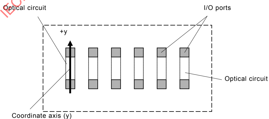
Figure 11 – Definition of direction of coordinate axis 2): Along a specific optical circuit (only if the wire is recognizable)
