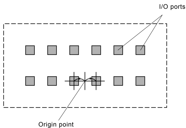
Figure 9 – Definition of origin point 2): Determination of an origin point at a place where there is no port (a mid-point of adjacent two ports at the centre of bottom line is used as the origin)
