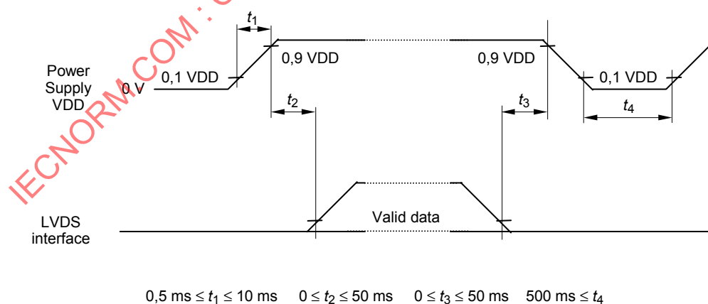
Figure A.3 – Logic power and LVDS signals sequencing diagram
