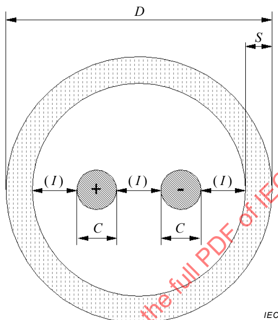
Figure 1 – Transverse section of simplex
