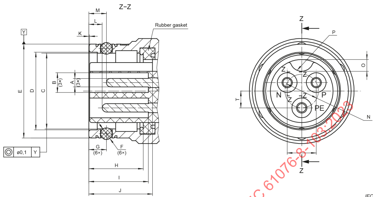
Figure 4 – Fixed connector
