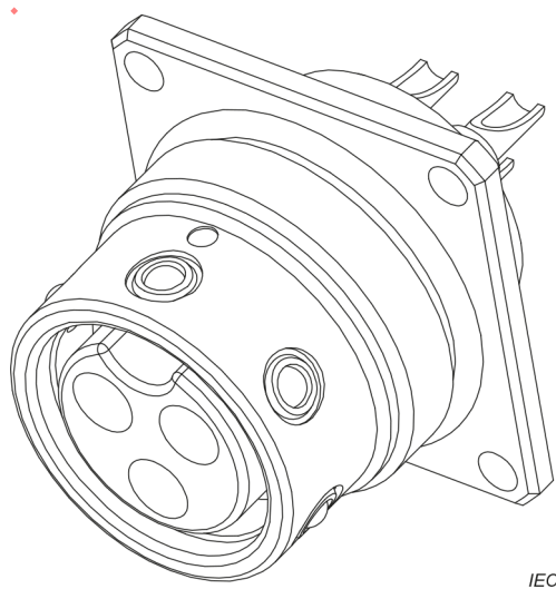
Figure 2 – Fixed connector
