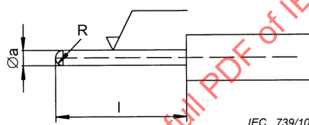
Figure 7 – Gauge dimensions
