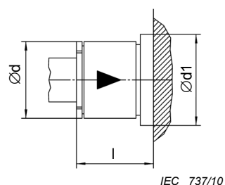
Figure 6a – Housing variant 1
