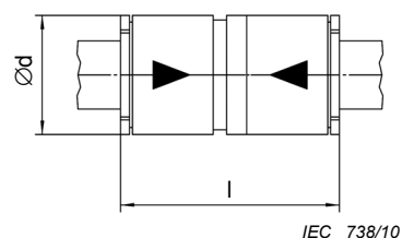
Figure 6b – Housing variant 2
