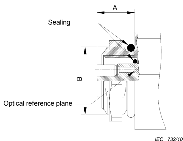
Figure 1 – Fixed connector, electrical female contacts, single hole mounting thread M16 \times 1,5 , mounting orientation
