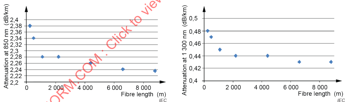
Figure E.2 – Example of attenuation coefficient tests on A1a.3 fibre
