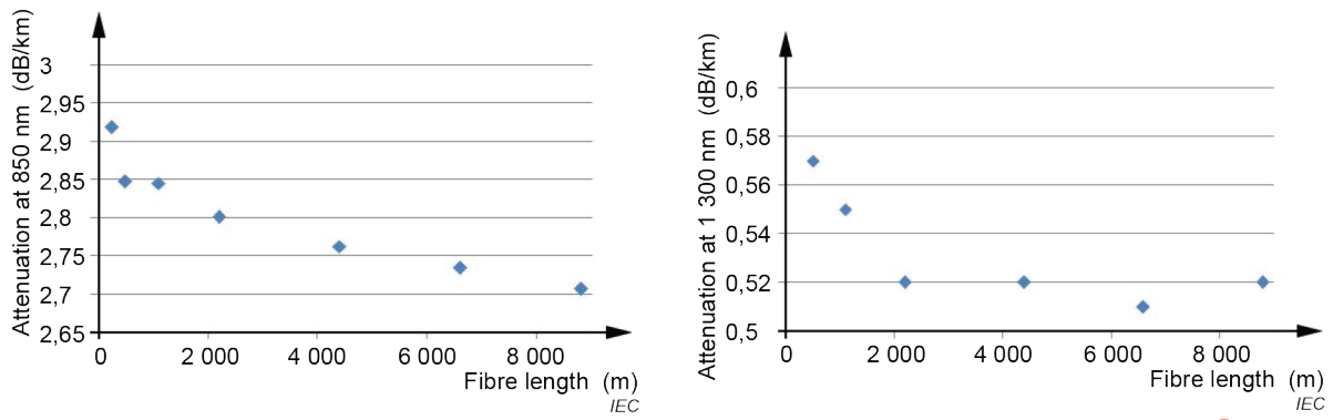
Figure E.3 – Example of attenuation coefficient tests on A1b fibre
