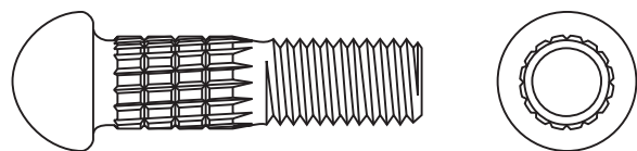
Bound-Body-Type High-Strength Bolt
