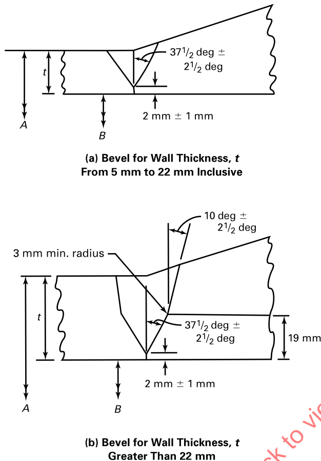
Figure 1 Welding Ends (Welding Neck Flanges, No Backing Rings)
